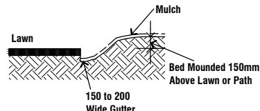
LAWN TO GERDEN BED DETAIL
