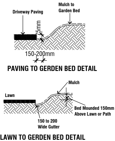
LAWN TO GERDEN BED DETAIL
