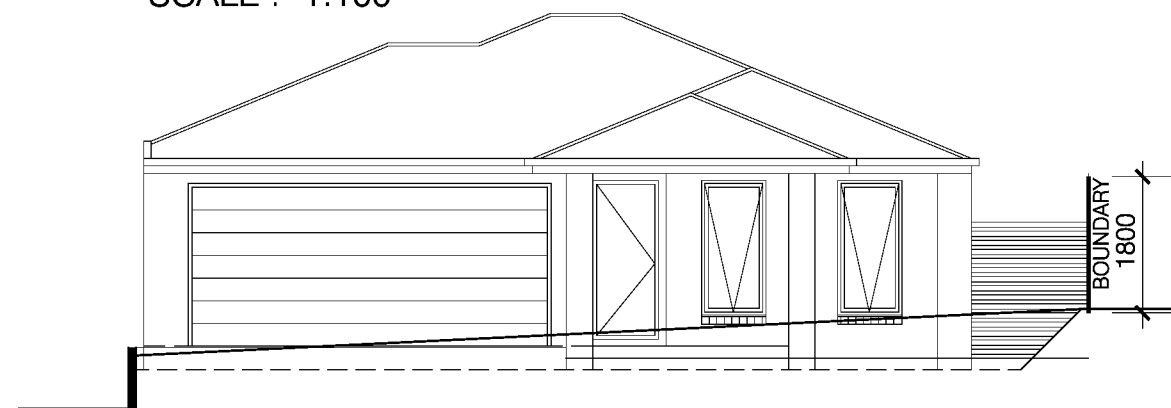
ELEVATION B EAST ELEVATION SCALE :- 1:100
