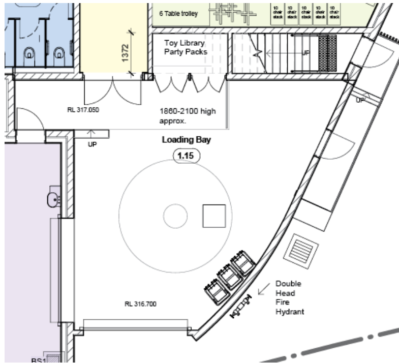
Storage within Loading Bay
